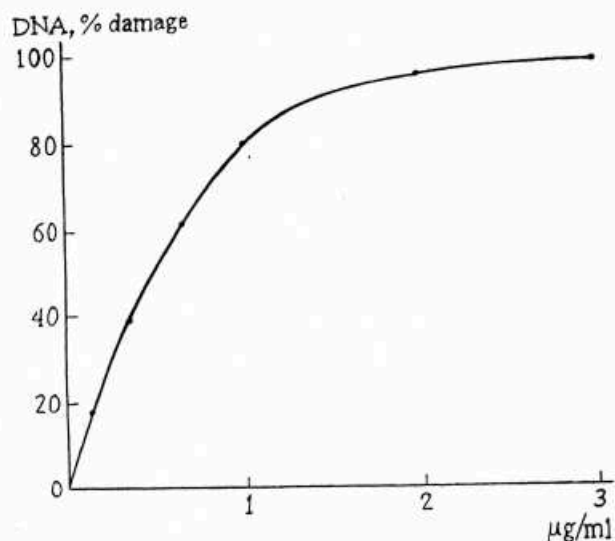
FIGURE 5. Effect of DA ( \times 10^{-5} \mu\text{M} ) concentration on the damage of \lambda DNA phage cross-linking (%).
