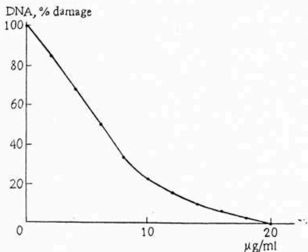
FIGURE 6. Effect of melanin concentration ( \mu\text{g/mL} ) on the damage of DNA (%) by products of peroxidase-catalyzed DA oxidation.
