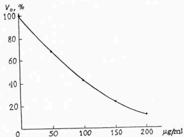
FIGURE 4. Effect of melanin concentration ( \mu\text{g}/\text{mL} ) on the rate of DA oxidation ( V_0 ).
