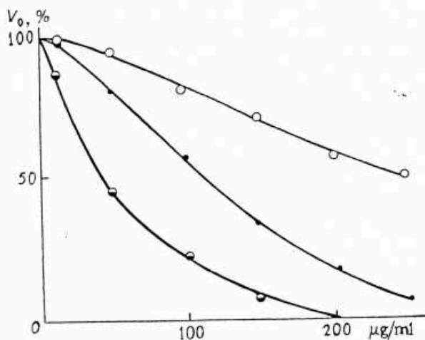
FIGURE 3. Effect of melanin concentration ( \mu\text{g}/\text{mL} ) on the rate of aminodiphenyl oxidation ( V_0 ): (1) benzidine; (2) 3,3'-dimethylbenzidine; (3) 3,3',5,5'-tetramethylbenzidine.
